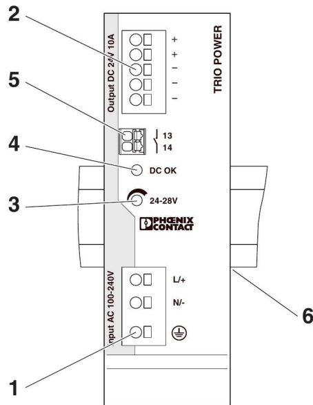
Figure 2 Function elements
