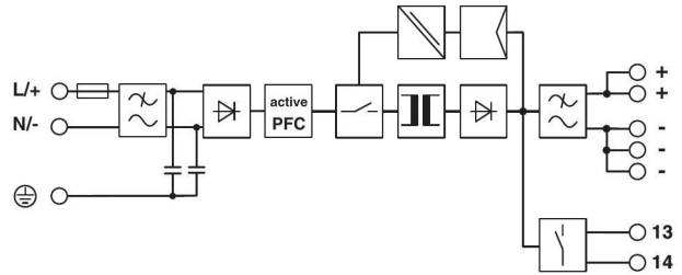
Figure 1 Block diagram
