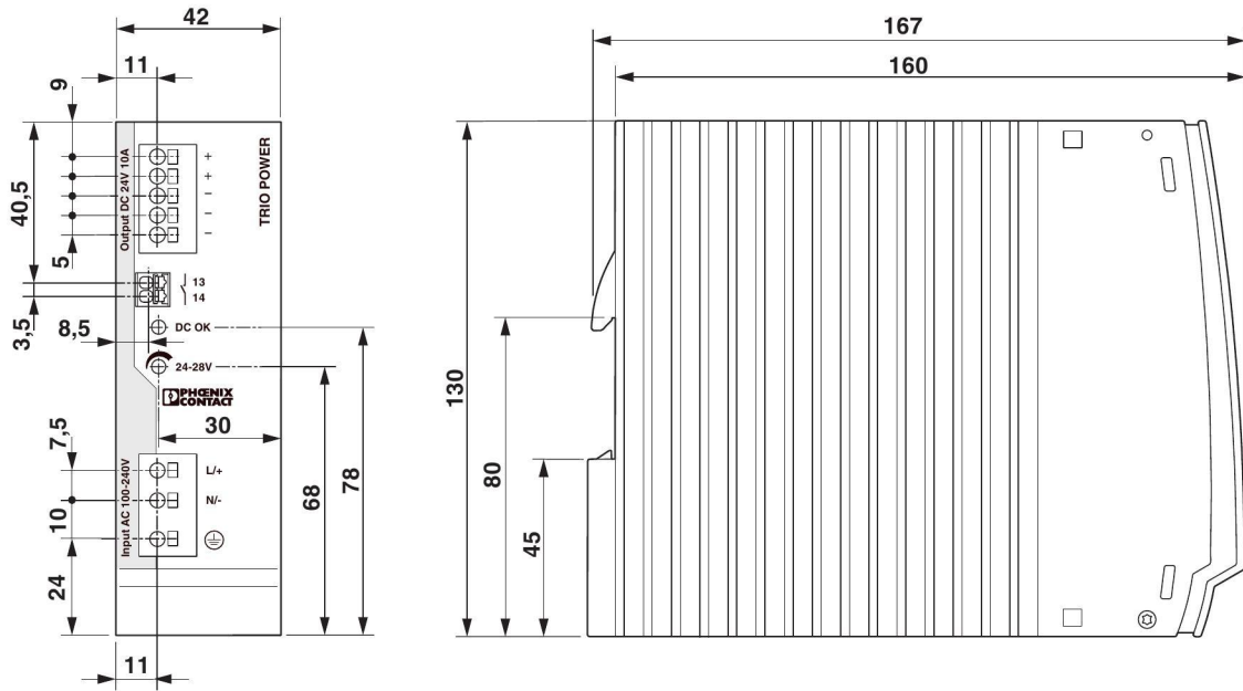
Figure 5 Device dimensions
