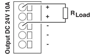
Figure 14 Schematic diagram, switching the output terminals
